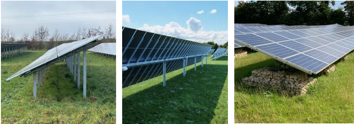
Figure 15-14 :Examples of Solar PV Generating Station Fixings
