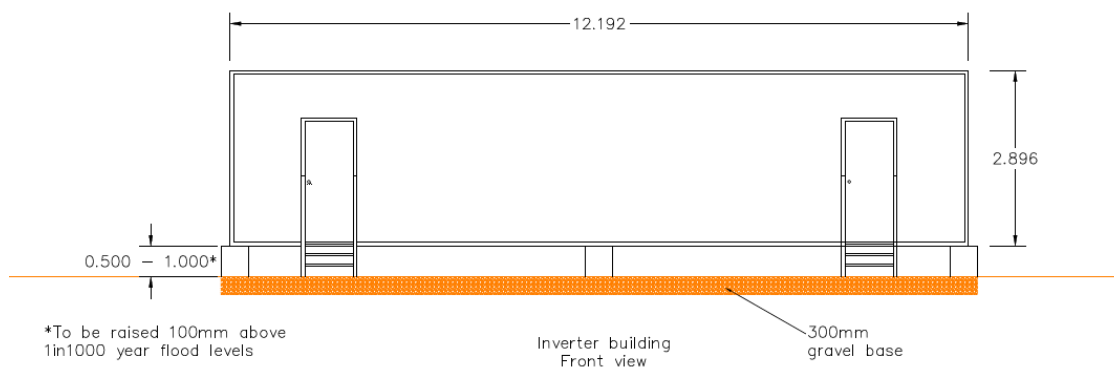
Figure 15-17: Typical Inverter Front Elevation
